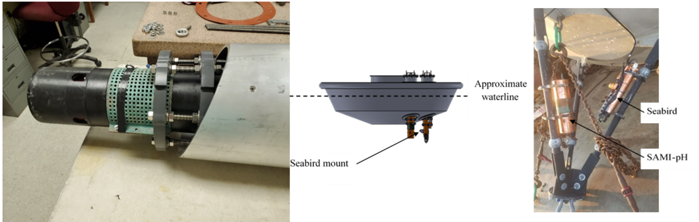
Figure 15. Comparison of existing buoy sensor deployment and proposed thru-hull configuration.
